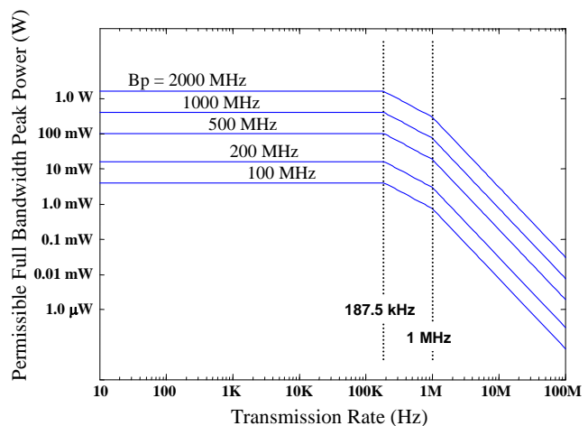
Fig. 1. Full Bandwidth Peak Power Constraint vs. Transmission Rate for Various -3dB Pulse Bandwidths.
